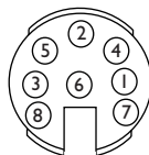
DC-iris Connector 8-PIN Female Connector (both viewed from solder side)
