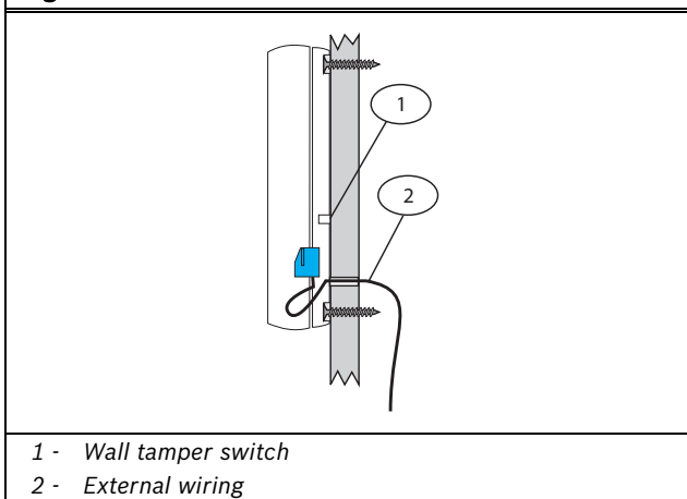
Figure 3: Mount the Transmitter on the Wall
