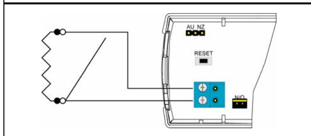
Figure 5: Wiring for Normally Open (N/O) Operation
