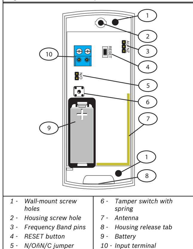
Figure 1: Transmitter Components
