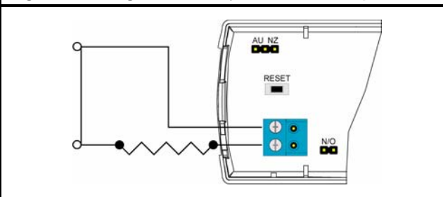
Figure 6: Wiring for Normally Closed (N/C) Operation
