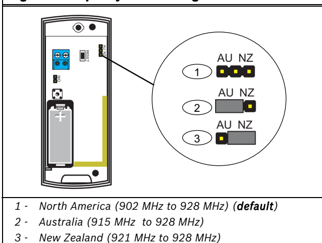
Figure 4: Frequency Band Settings
